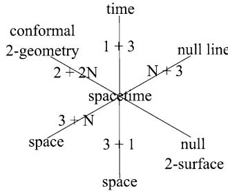
Fig. 36.1 There are 3 types of split depending on whether 0, 1 or 2 null directions are involved. While could be used in place of space or time directions, passing to null directions while leaving the time direction untouched causes additional complications and is not usually attempted. Primality can also be ascribed to each of the six entities in the figure in turn. Each of the six notions depicted as vertices has its own space of spaces, and each edge in the diagram has corresponding maps running in both directions. In these ways, the current Chapter’s considerations substantially increase the number of Problem of Time facets. Whereas the 2 instances of space in the diagram are the same object, the associated PDE systems are different in the case of each split
