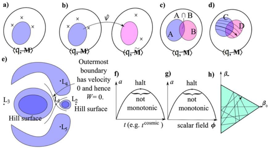
Fig. 37.1 a) PoZIN type restriction to a region. The crosses denote points at which zeros, infinities or non-smoothnesses of \mathcal{W} occur. b) PoZIN type restriction applying due to the domain of definability of a function thereupon, e.g. for \psi a conformal transformation. c) With different approximations used in general having different domains of validity, an intersection in which all of them are valid is a smaller domain. d) Patching constructs extend from a region C in which one set of approximations applies to a partly overlapping region D in which some other set of approximations apply; see Sect. 59.2 for a well-known example of this. e) Equipotentials for the Earth–Moon–Sun system, illustrating Hill’s regions, as an example of PoZIN being realized in a physically relevant model. The L_i here are the well-known Lagrange points . f) Closed recollapsing FLRW universe scalefactor; g) is a relational version of this. h) Bianchi IX’s sequence of potential zeros; the straight line segments correspond to Kasner solution ‘in’ and ‘out’ states being scattered by the Bianchi IX potential
