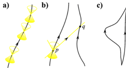
Fig. 4.3 a) Worldline concept, presented with decoration by null cones at each of its points. For extended objects, worldsheets, worldvolumes... are defined similarly. b) Worldlines 1 and 2 with event p on worldline 1 able to influence event q on worldline 2. c) The worldlines for the twin ‘paradox’, and the naïvely symmetric situation that does not actually model the physics experienced by the two twins
