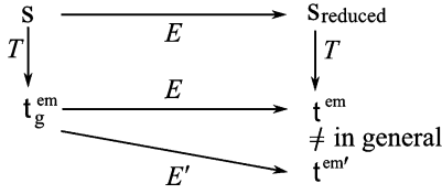
Fig. 18.2 Let us denote the map from an action to the corresponding emergent time candidate by T , We denote the map consisting of substituting in the \mathfrak{G} -extremum of the action by E , and the map consisting of substituting in the \mathfrak{G} -extremum of the timefunction itself by E' E and T naturally commute: TE = ET , but in general TE' \neq ET . This is why we use the \mathfrak{S} -extremum of \mathfrak{S} in order to free t of \mathfrak{g} -dependence
