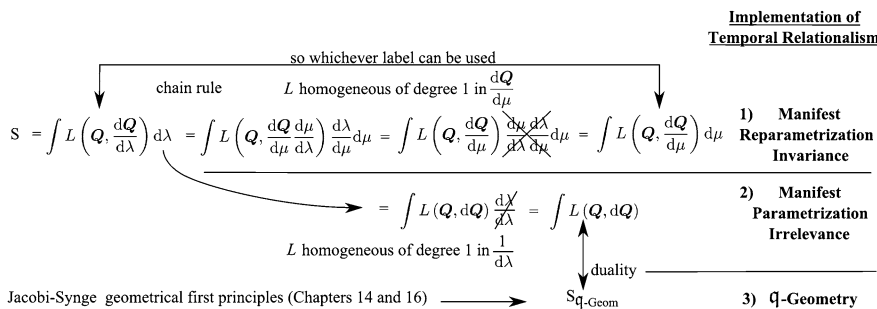
Fig. 9.2 Inter-relation of this book’s three implementations of Temporal Relationalism at the level of actions
