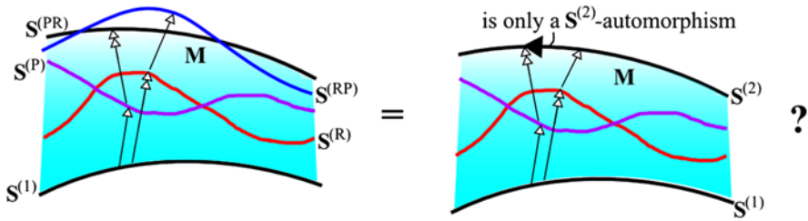
Fig. 38.4 Reslicing Invariance posed. Consider the larger notion of mathematical space M in the role of spacetime and the smaller notion of mathematical space S in the role of space. Is the solid arrow's transformation due to difference between passing from S^{(1)} to S^{(2)} via the red and purple intermediate S's always an automorphism of S^{(2)} ?
