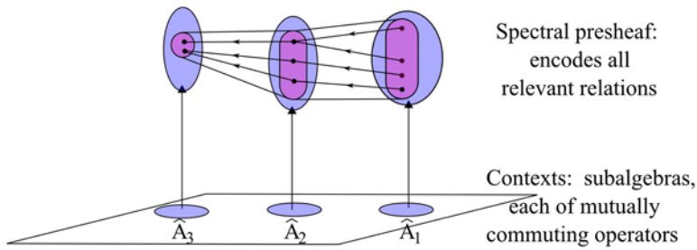
Fig. W.4 Example of a topos presheaf construct, as used in formulating the Kochen–Specker Theorem. This figure illustrates that not all cases within a given floor of the tower can be extended up the tower
