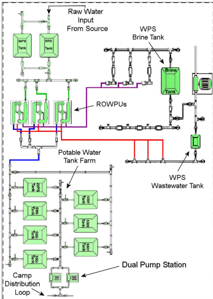
Figure 8.6. Typical Water Production Subsystem Layout.
