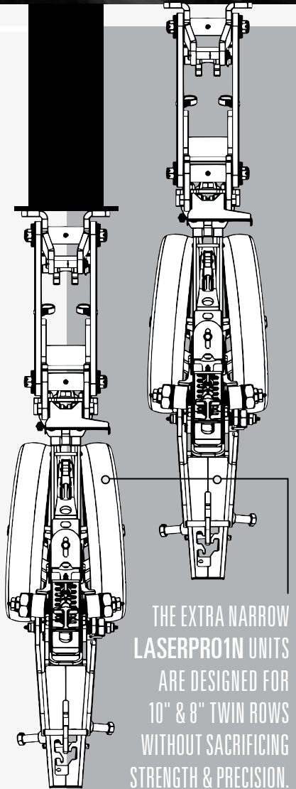
LASERPRO1 w/ vDrive insecticide boxes Integrated with FurrowJet.
