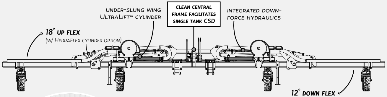
SB4036-TR ULTRALIFT™ 36" TWIN ROW LASERPROIN-TR W/ 1.2BU HOPPERS
