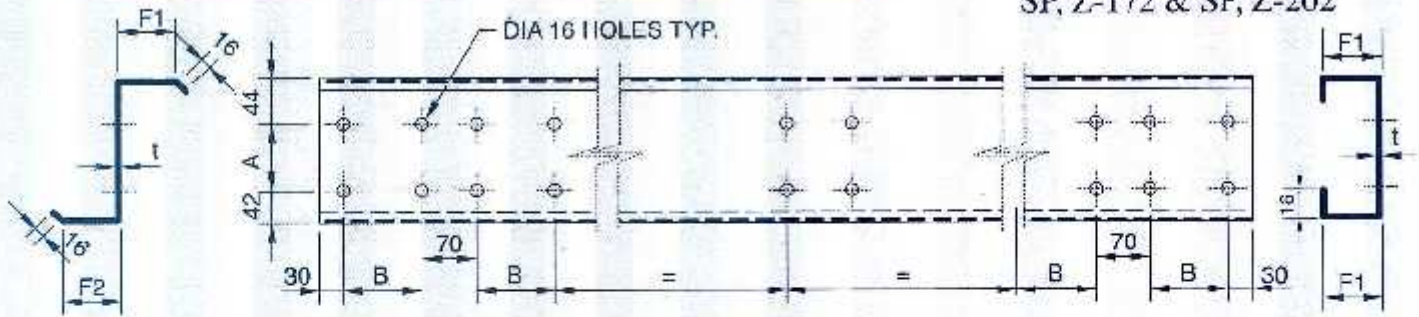
PURLIN SECTION & ELEVATION
