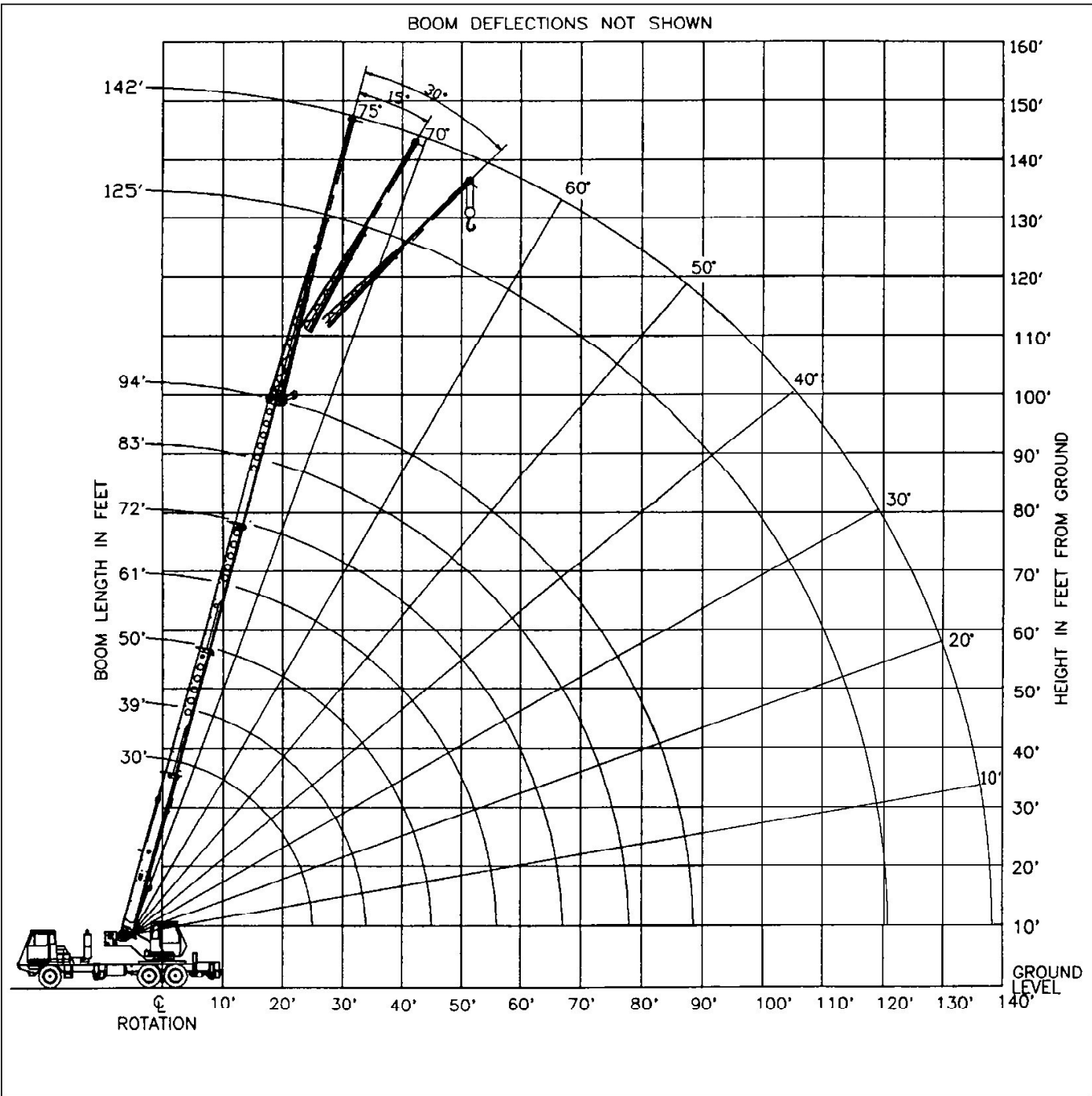
Range Diagram (30' - 94' boom)
