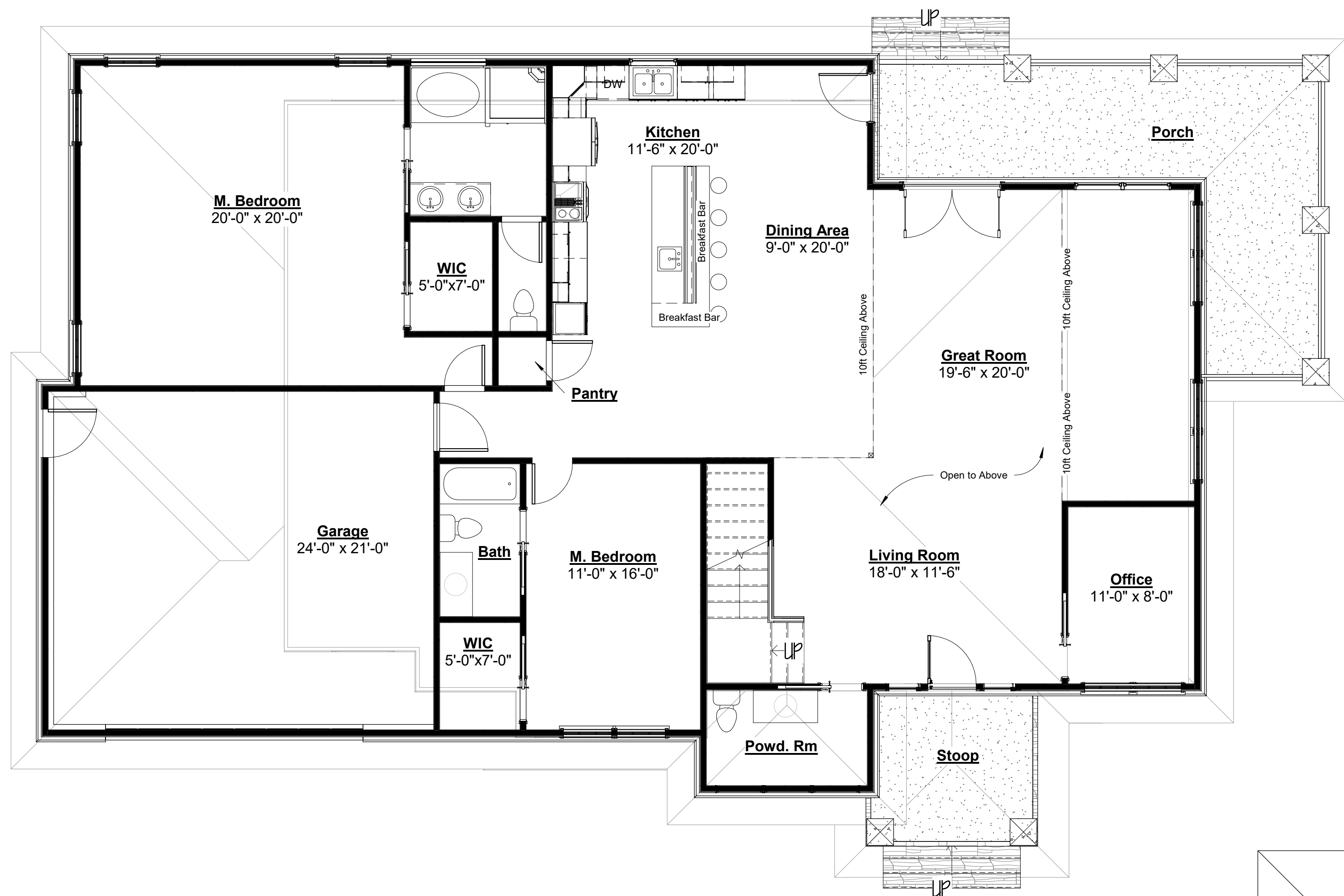
1 First Floor Prelim 3/16" = 1'-0"
