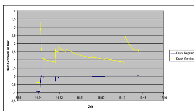
Dynamic flow profile by use of pro-active direct infusion into mould
