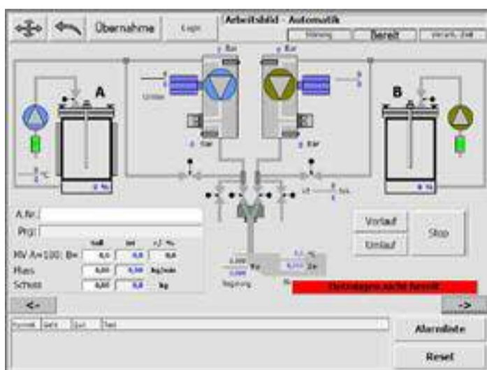
Dynamic flow profile by use of pro-active direct infusion into mould
