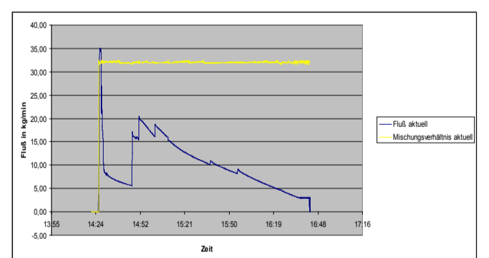
Dynamic flow profile by use of pro-active direct infusion into mould
