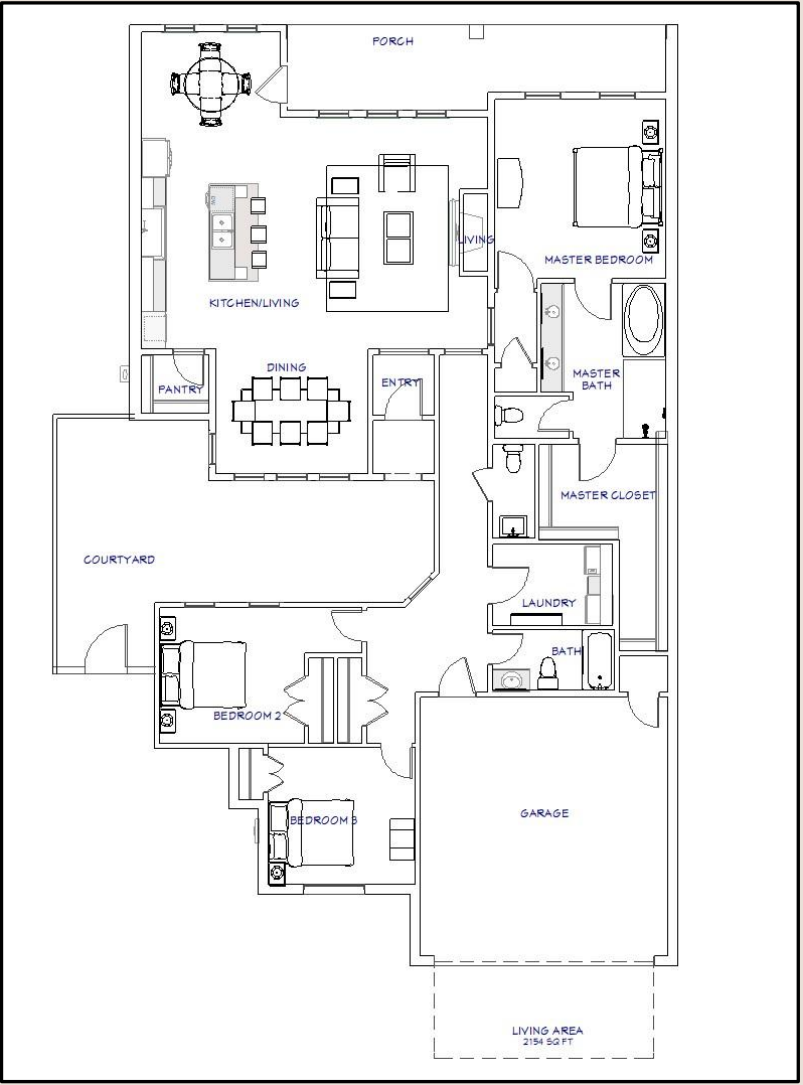
BASIC PLAN
