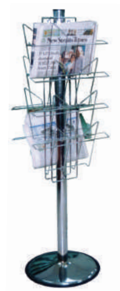
NAGA 060 CHROME FINISHED NEWSPAPER DISPLAYER 381 Diameter x 1524H mm
