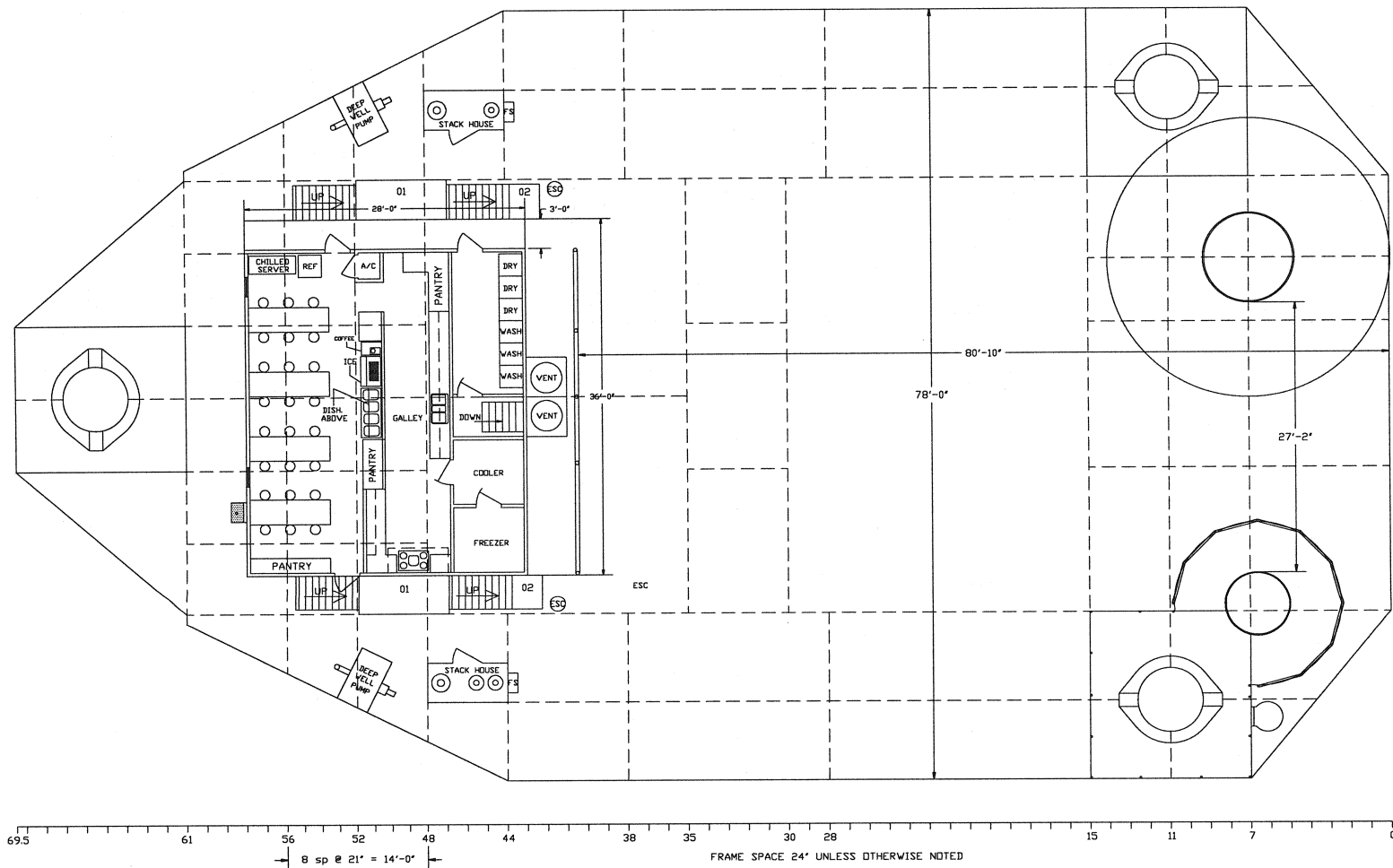
GENERAL ARRANGEMENT MAIN DECK
