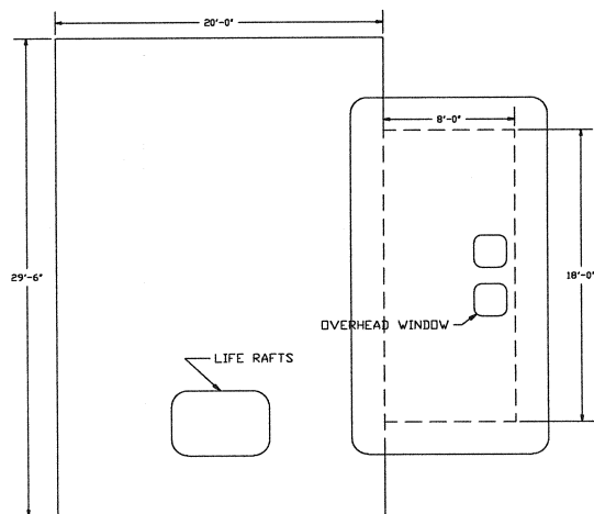
GENERAL ARRANGEMENT 04 LEVEL SCALE 1/4" = 1'-0"
