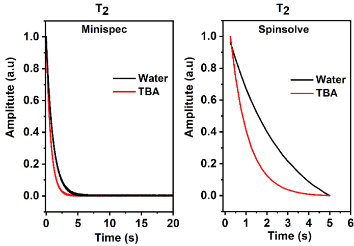
Figure 2. Spin-spin spectra for the Minispec and Spinsolve devices
