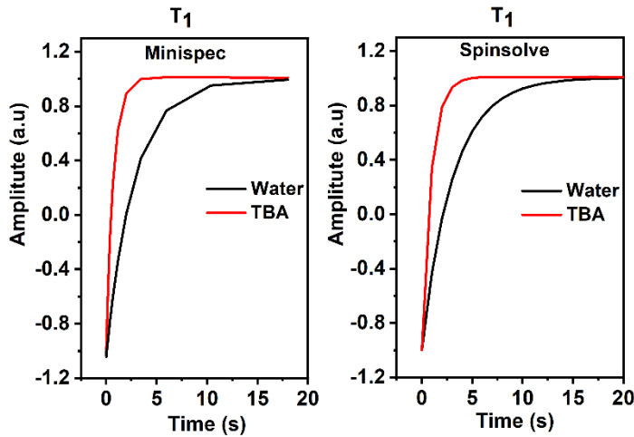
Figure 3. Spin-lattice spectra for the Minispec and Spinsolve devices
