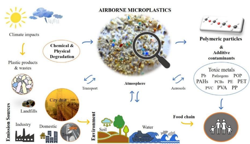
Figure 1. Sources, formation, and circulation of atmospheric microplastics in the environment.
