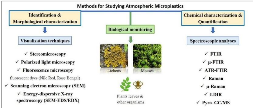
Figure 2. Diagram of analytical techniques and biomonitoring methods.
