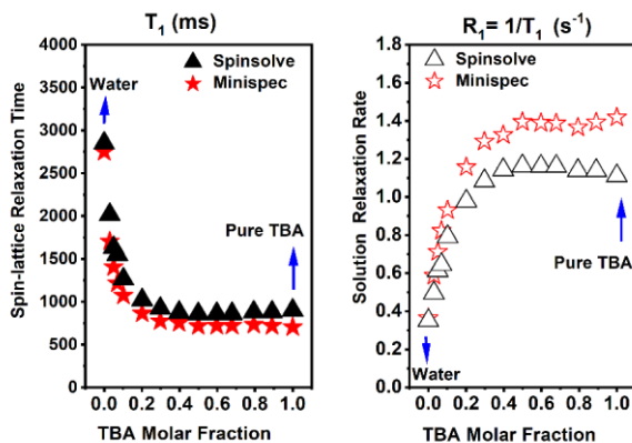
Figure 5. Spin-lattice and relaxation rate times for the mixture.
