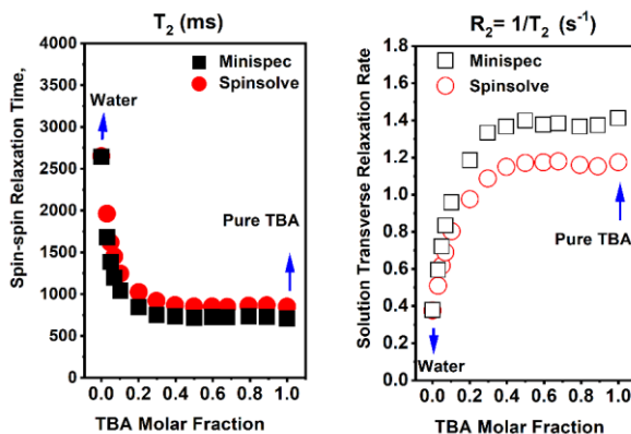
Figure 4. Spin-spin and relaxation rate times for the mixture.
