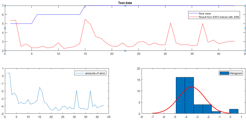
Figure 4: The graphics of the results from ANN trained with SWO on glass test data (for n=100 )
