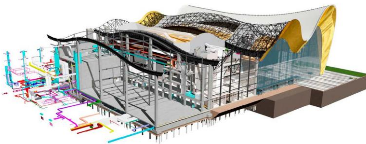
Figure 8. Combination of models prepared by different disciplines (Pride, 2025)
