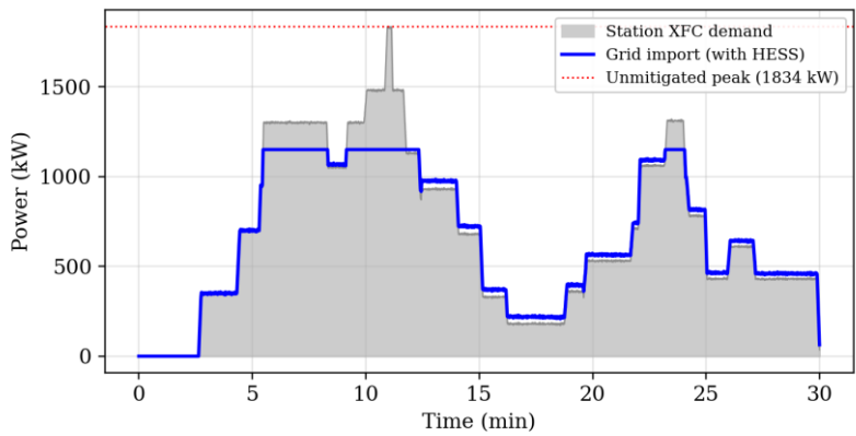
Figure 1. Station XFC demand and the resulting grid import with HESS peak shaving; the grid is held at the 1150 kW contractual cap during peaks.
