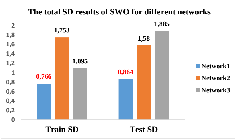
Figure 18: The graphics of total train and test SD results of SWO for different networks
