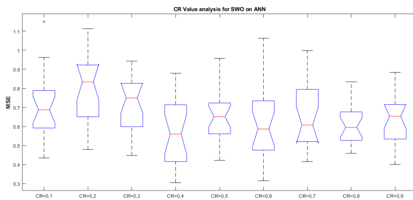
Figure 14: The boxplot of the CR value analysis for SWO on ANN
