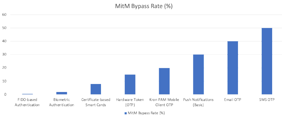
Figure 2. MitM Bypass Rates Against MFA Methods
