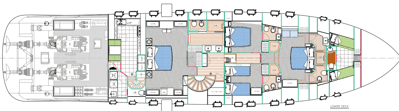
LOWER DECK
