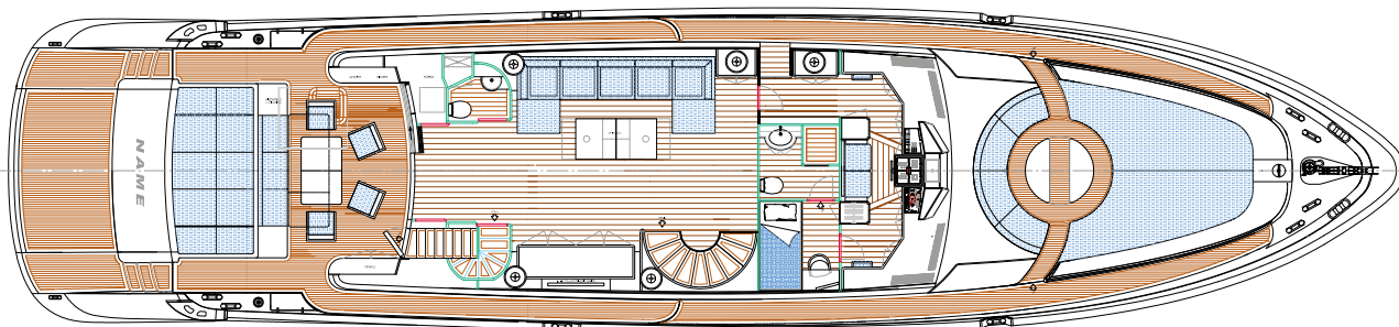
MAIN DECK
