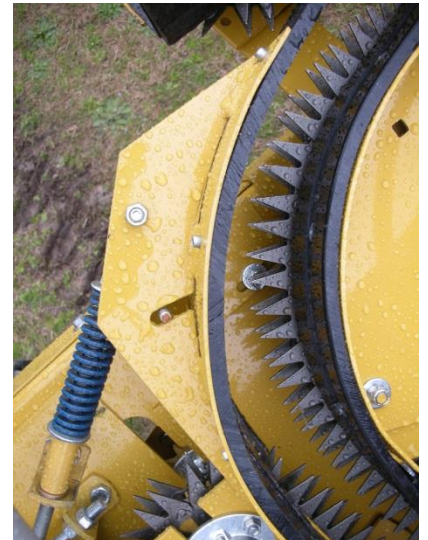
Spring loaded transition for varying stalk sizes
