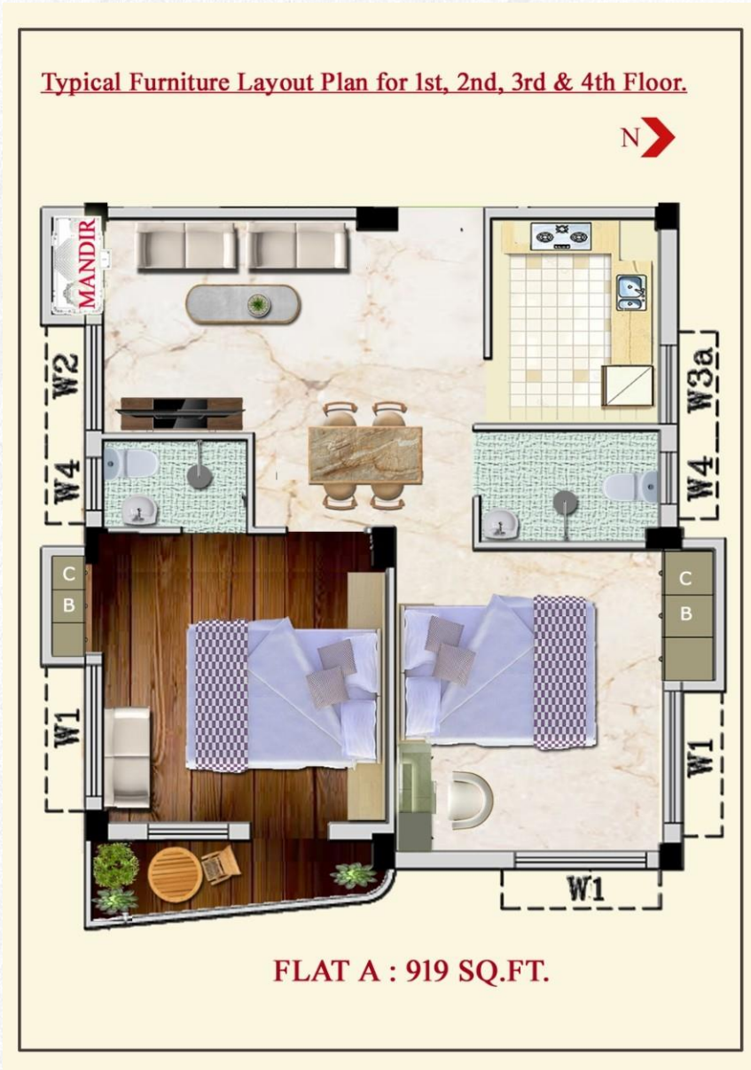
1st To 4th FLOOR PLAN
