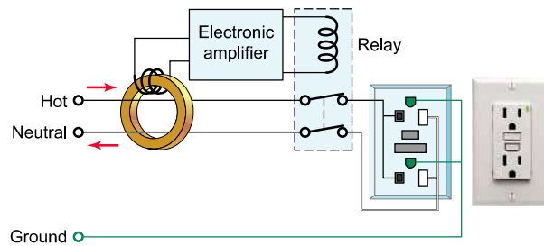
Figure 1-9 GFCI receptacle.
