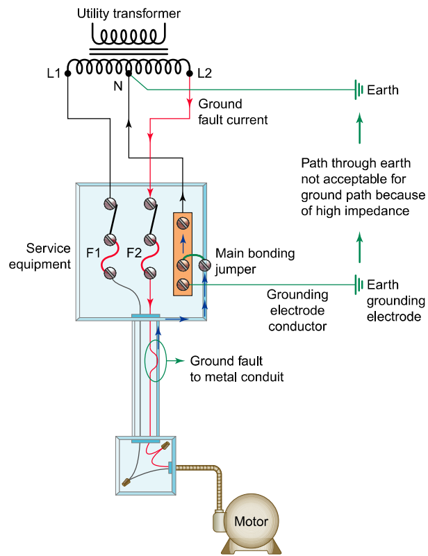
Figure 1-7 Ground-fault current path.
