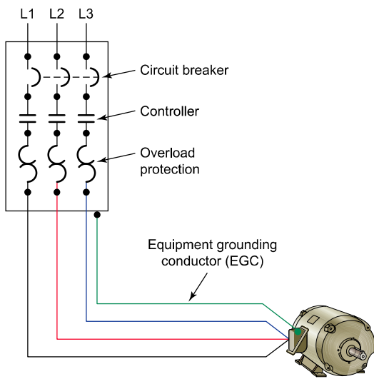
Figure 1-8 Equipment grounding conductor (EGC).
