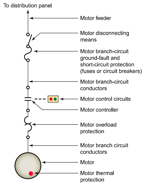
Figure 1-12 Motor terminology.
