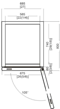
C-23RM TOP VIEW
