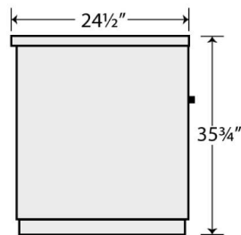
SIDE VIEW (1,2,3 DOORS)
