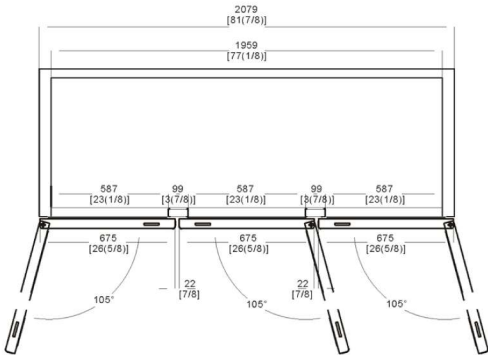
C-72RM TOP VIEW
