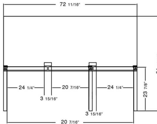
C-U72R TOP VIEW
