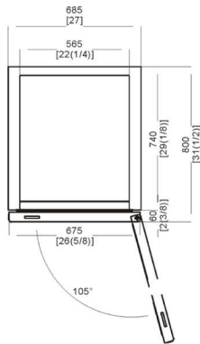
C-23FM TOP VIEW
