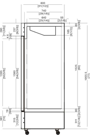
SIDE VIEW (1,2,3) DOORS MODELS
