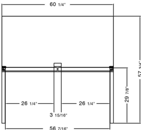
C-U60F TOP VIEW
