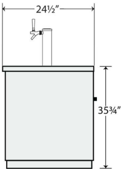
SIDE VIEW (1,2,3 DOORS)
