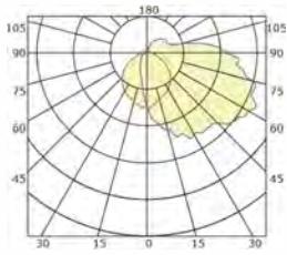
Average Diffuse Angle(50%): 103.0°
