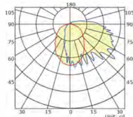
Average Diffuse Angle(50%): 93.0°
