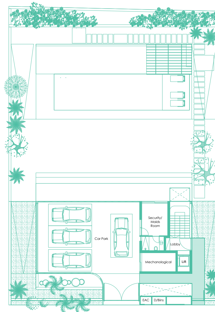
Second Floor 46 s.m.
