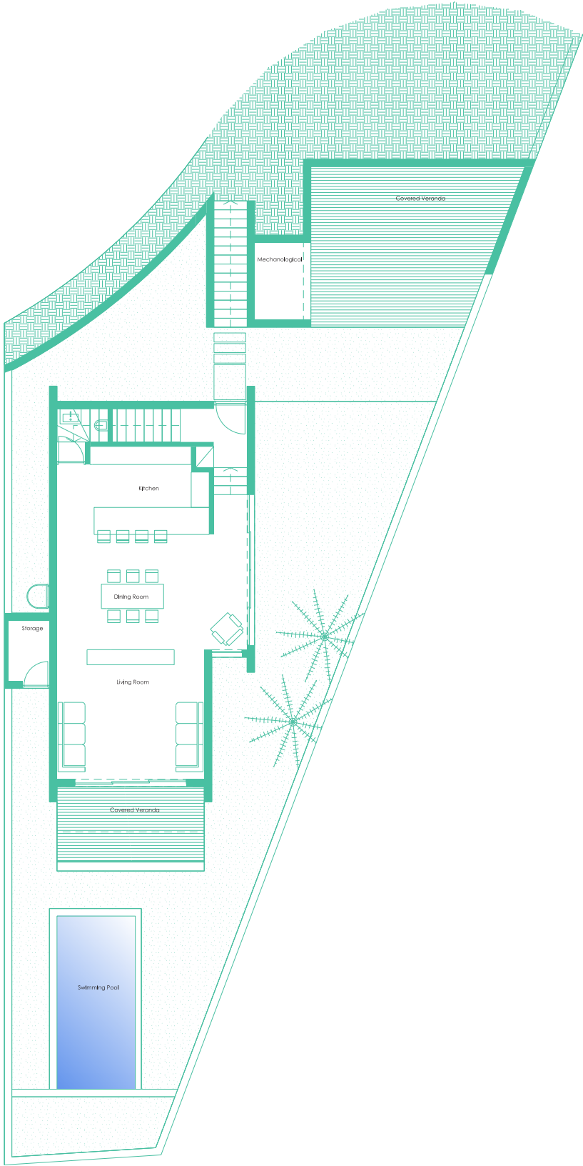
Ground Floor 85 s.m.
