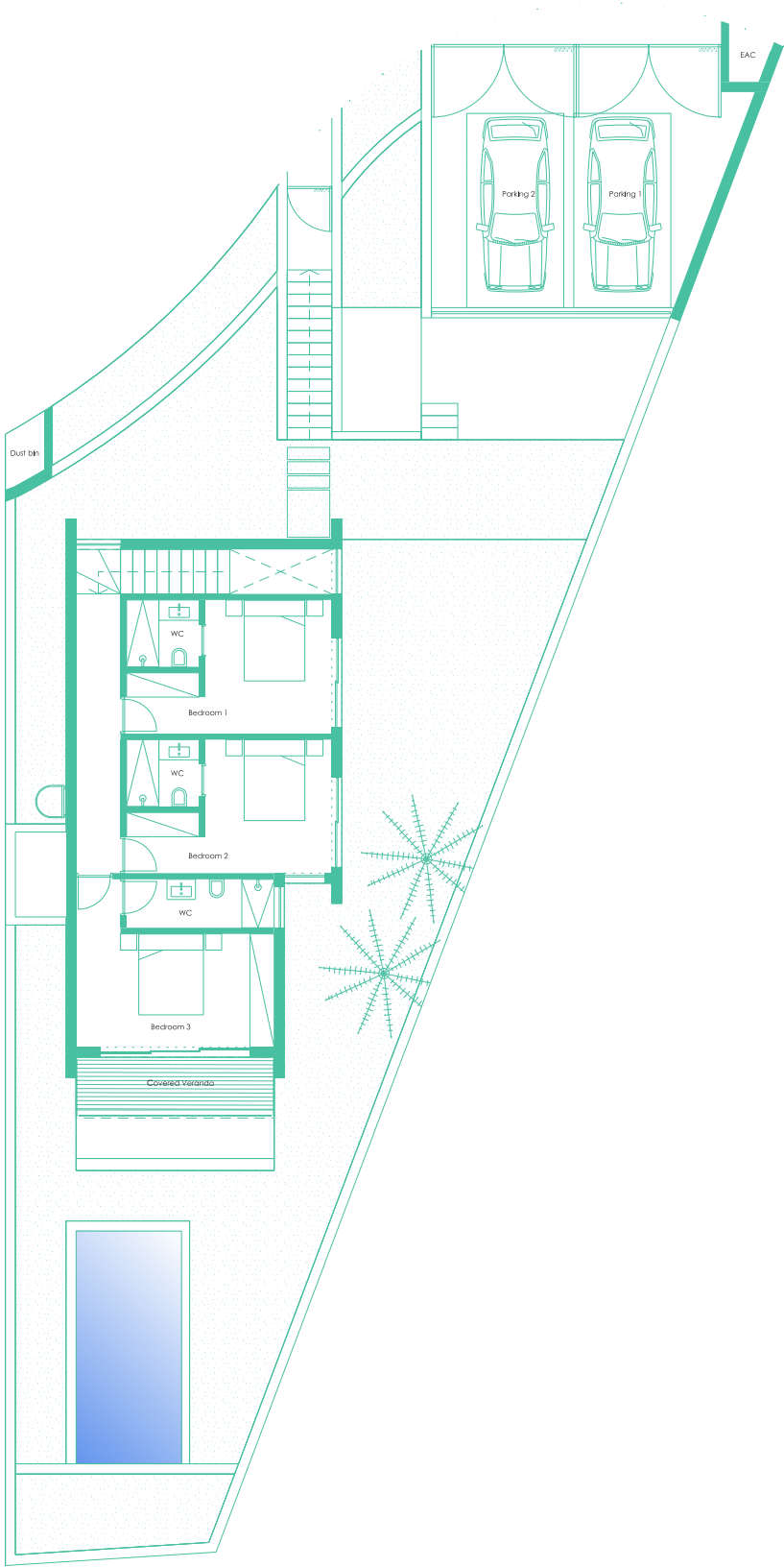
First Floor 85 s.m.
