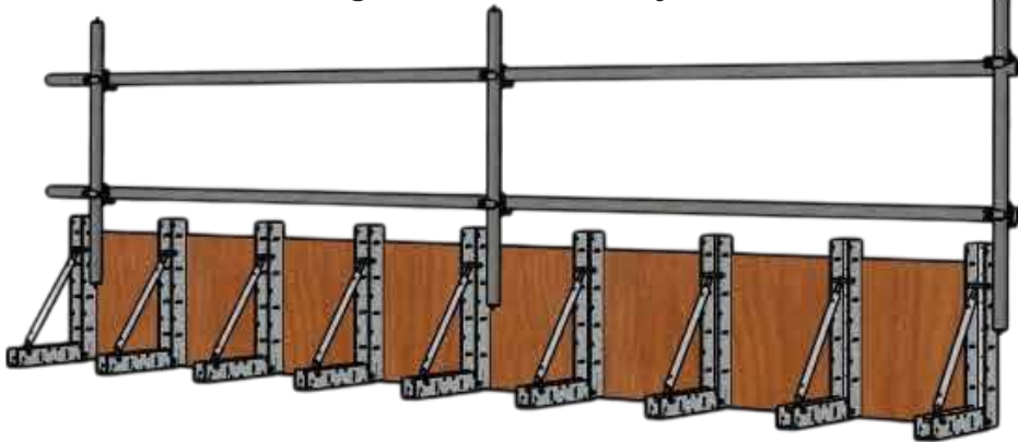
Slab edge with handrail, ability to attach tube & fitting or Combisafe style handrails
