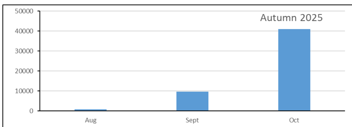
Figure 7. Number of registered birds by months during the autumn migration in the territory of ISPB.
