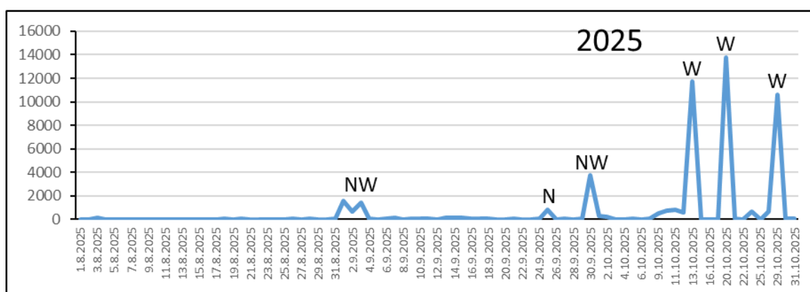
Figure 8. Dynamics of the autumn migration of the flying bird species in the ISPB territory according to visual observations during the period 01 August - 31 October 2025. Letters indicate the direction of wind in days with increased number of migrating birds.
