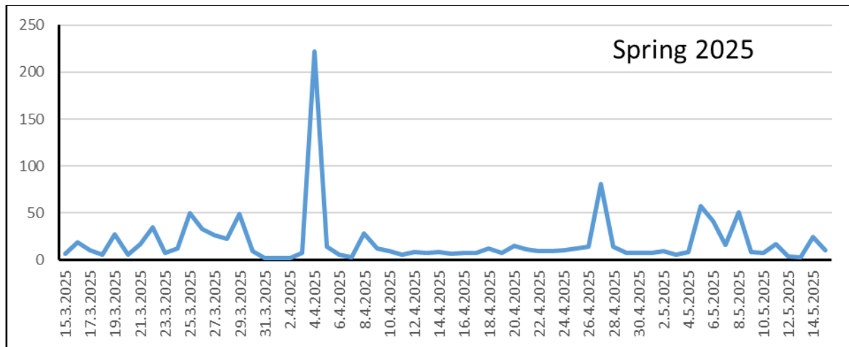
Figure 6. Dynamics of the spring migration of birds in the ISPB territory based on visual observations during the period 15 March - 15 May 2025
