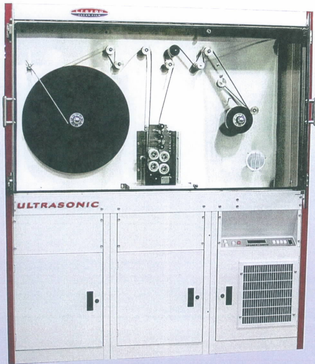
Shown above...the 6000 Foot Capacity Model CF9206 which is also available for use with HFE-8200 or perchloroethylene solvents
