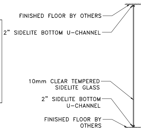
TYPICAL SIDELITE SECTION
