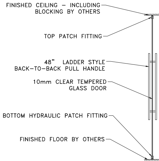
PATCH FITTING DOOR SECTION
