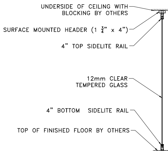
TYP. ENTRY SIDELITE SECTION
