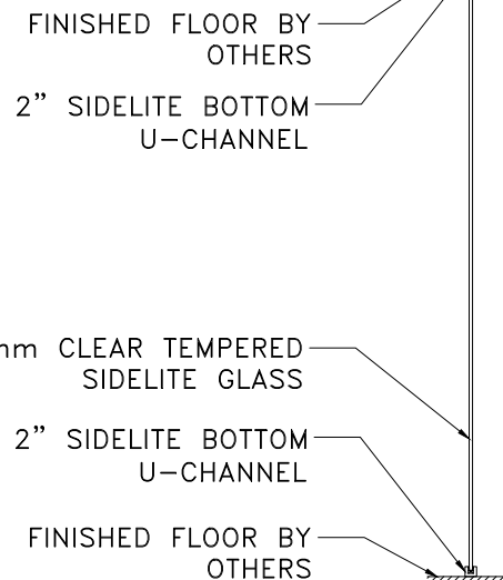
TYPICAL SIDELITE SECTION
