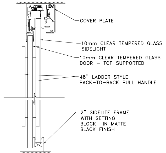
1 FH SLIDING DOOR & TRACK SECTION
