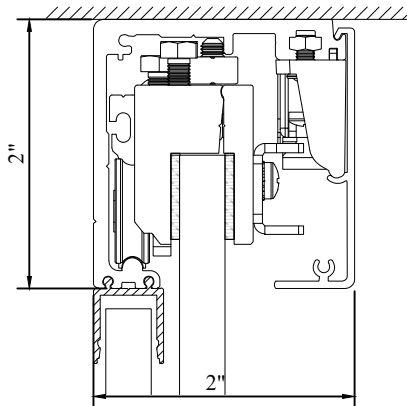
FH SLIDING DOOR PROFILE SECTION
