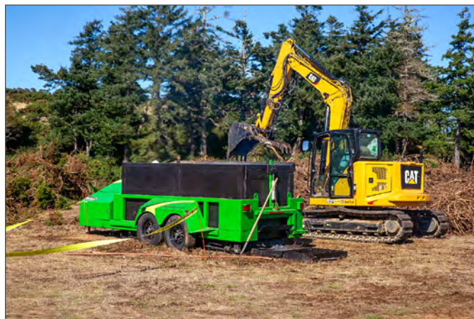
Figure 2.1. This biochar production unit 1 and loader are an example of moderate-scale biochar production. Here, biomass resulting from removal of invasive gorse is converted to biochar in Bandon, Oregon. Conversion to biochar inhibits the spread of the invasive plant. (Photo: U.S. Forest Service Region 6 State & Private Forestry)
