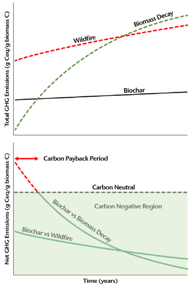
Figure 1.4. Two stages in a hypothetical time-sensitive LCA of biochar technology. (Top) Total GHG emissions of biochar and two alternative fates of the same woody biomass feedstock (decay in place and wildfire). (Bottom) Net GHG emissions of the biochar approach relative to biomass decay and to wildfire. The C-payback period is the period during which biochar technology has higher cumulative GHG emissions than the biomass-decay option.
