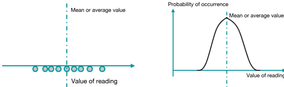
Figure 7: Distribution of readings
