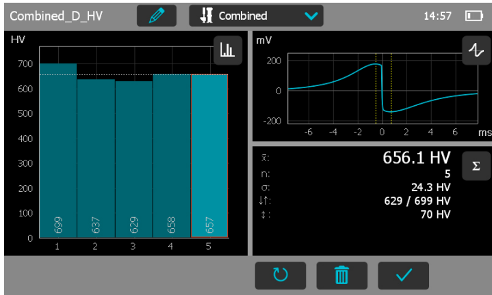
Figure 27: Equotip 550 after five performed measurements
