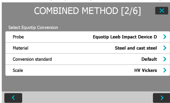
Figure 23: Screenshot of settings for the Leeb measurements
