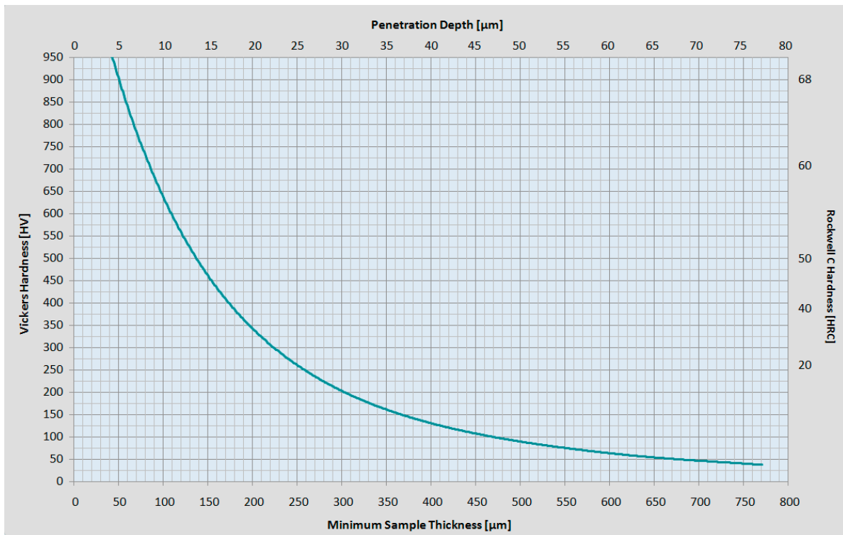
Figure 6: Portable Rockwell conversion curve
