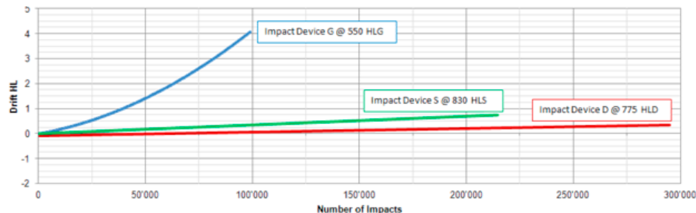
Figure 11: Drift of measurement values in relation to number of impacts performed.
