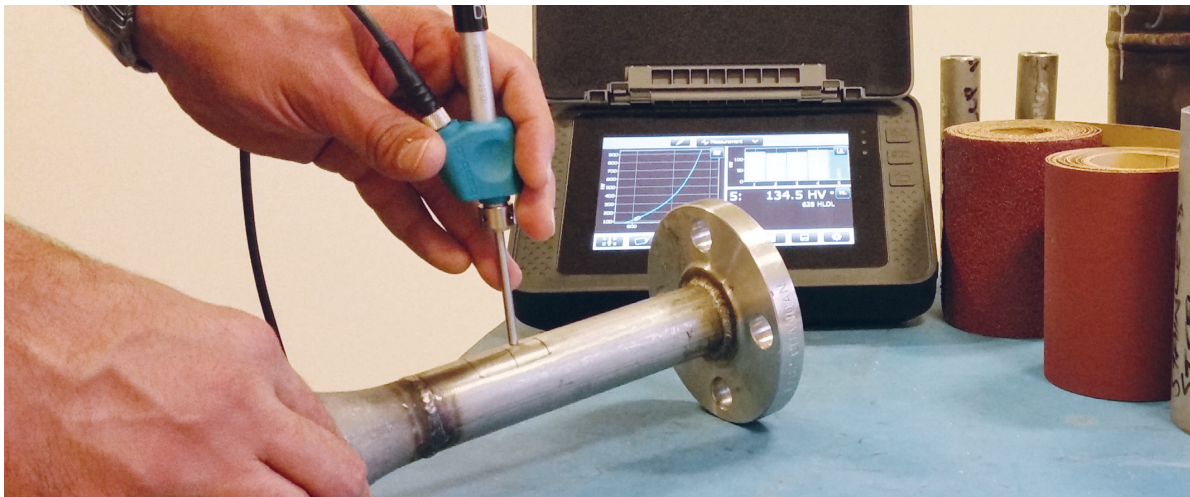
Figure 26: Performing Leeb measurements on test sample
