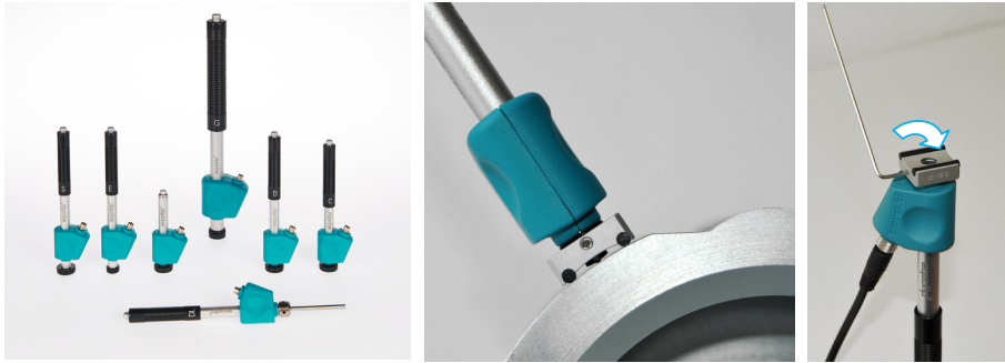
Figure 12: Overview of Equotip 550 Leeb Impact Devices and usage of support rings
