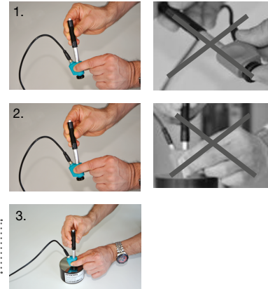
Figure 8: The Leeb measurement procedure in three steps.
