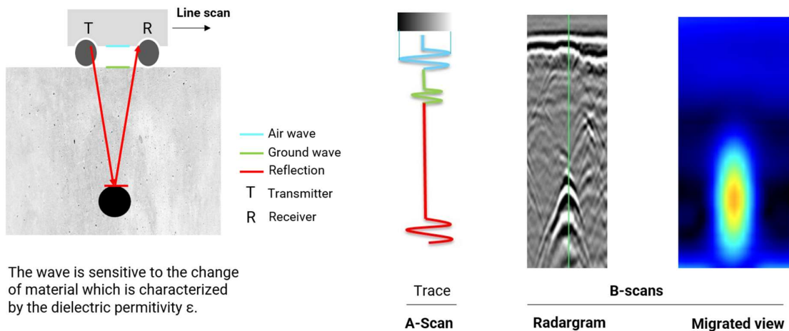
Figure 13 : A-scan, B-scan & migrated views principles
