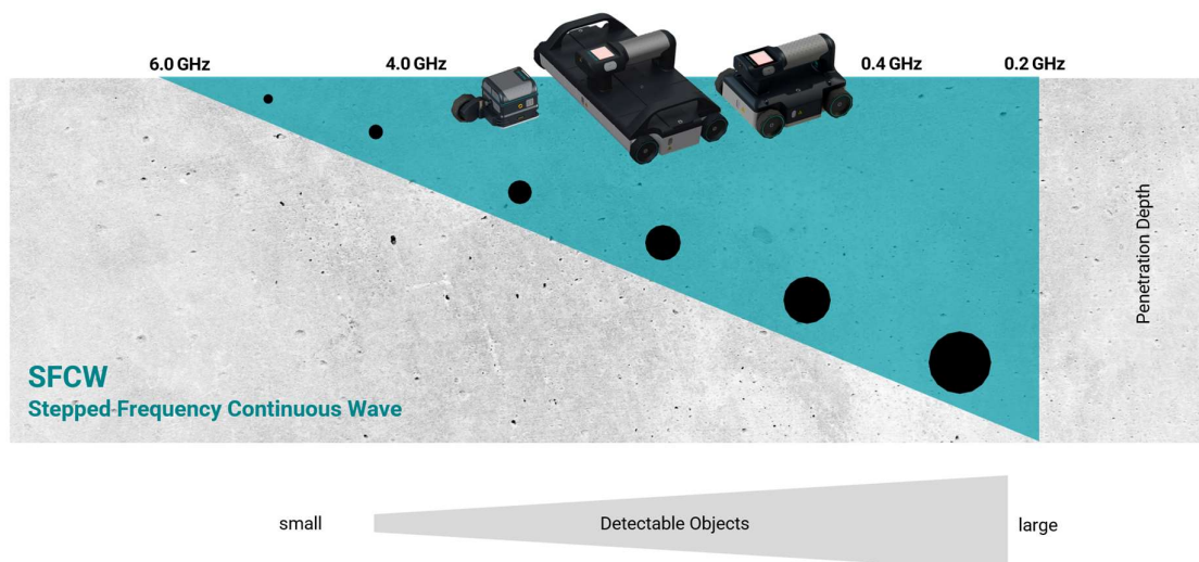
Figure 4: Stepped-Frequency-Continuous-Wave principle
