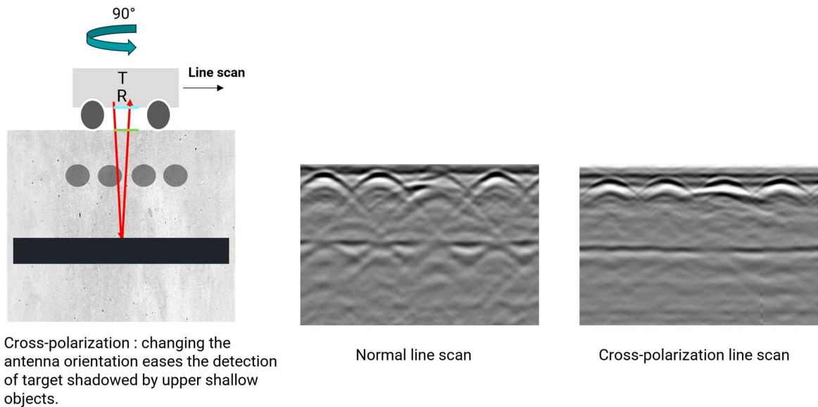
Figure 16: Cross polarization principle
