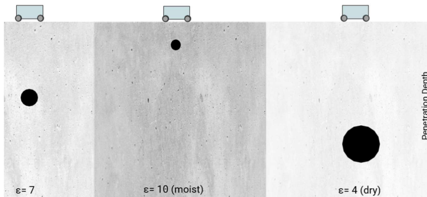
Figure 31: Concrete dielectric \epsilon principle
