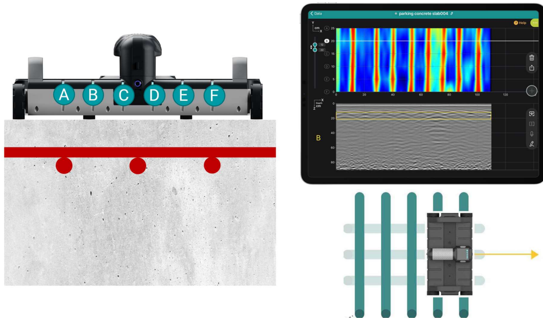
Figure 18: GP8100 Superline scan
