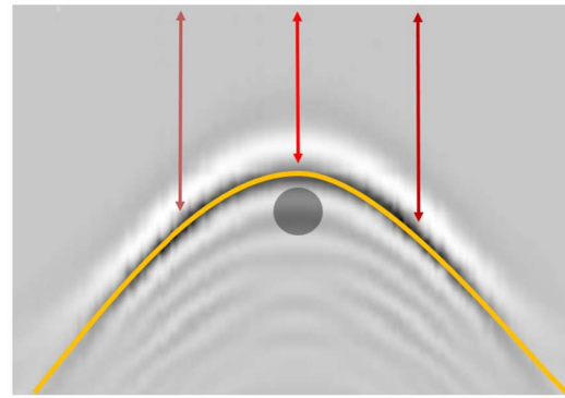
The wave reflects back at distances forming an hyperbola.
