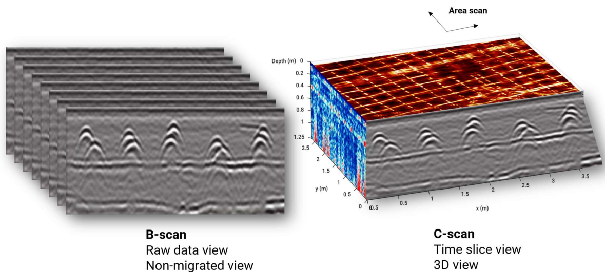
Figure 19: Area scan, 3D view & time slice view principle
