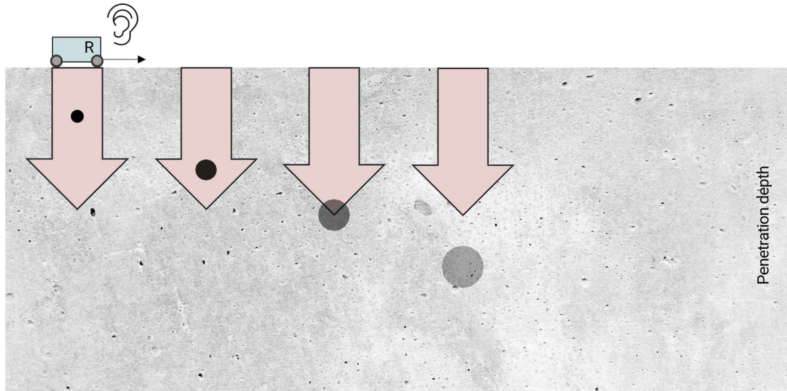
Figure 34: Time window principle
