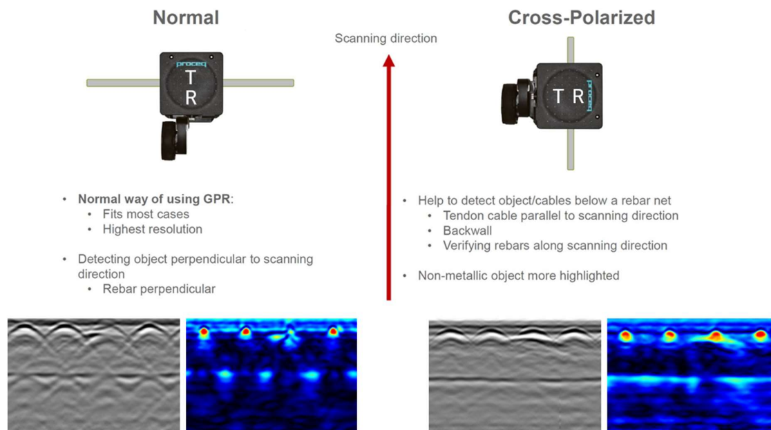
Figure 17: GP8800 Cross polarization setting
