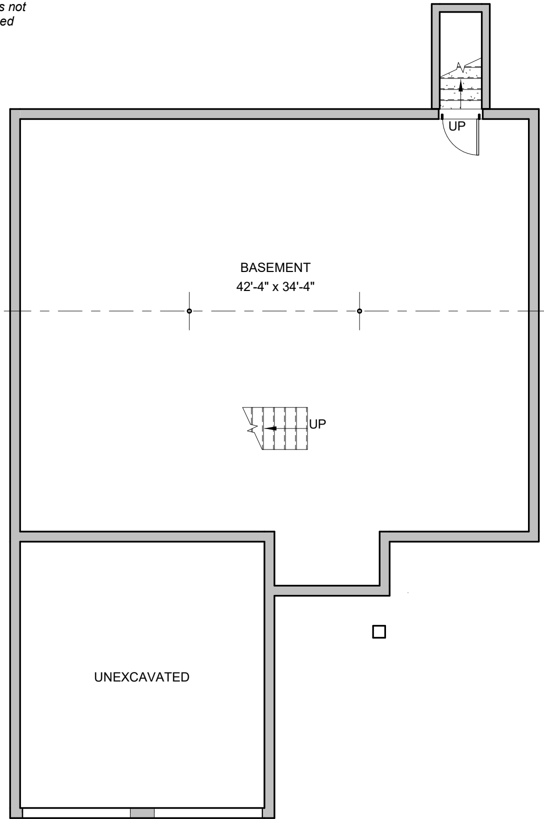
BASEMENT PLAN 1,629 gsf (unfinished)
