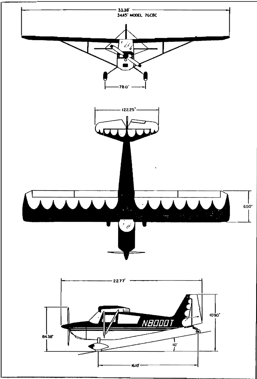
FIGURE 6-2 CITABRIA THREE-VIEW
