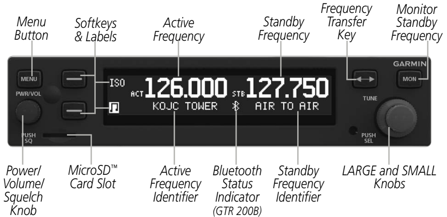
GTR 200/200B Front Panel
