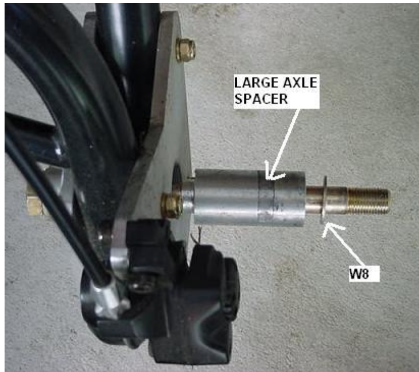
Figure 18 – Outside Axle
