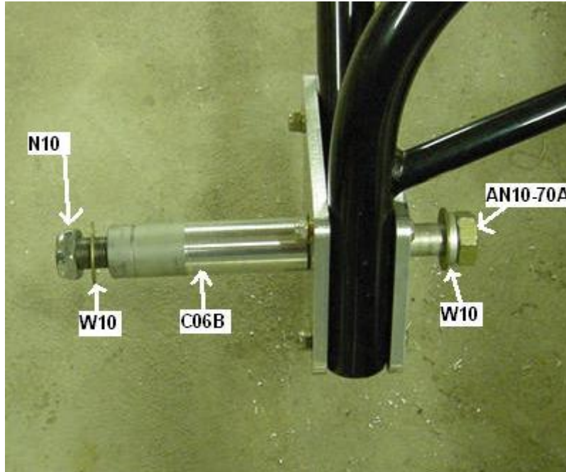
Figure 20 – Washer and Bolt Spacing
