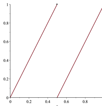
Figura 2: “Doubling map”
