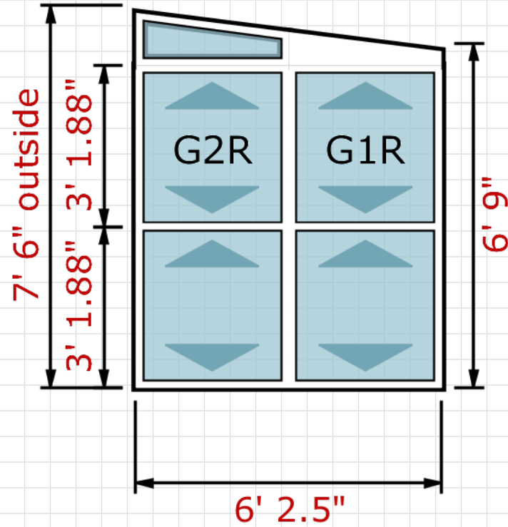
RIGHT END - WIDTH
