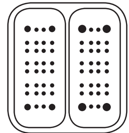
FL*-64A 8 - Size 16 56 - Size 20
