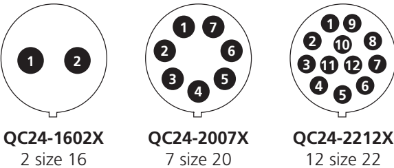
Receptacles - cavity identification from rear
