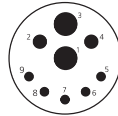
24-91 2 size 8, 2 size 12 & 5 size 16 N, E
