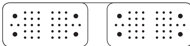
DRC20-76P*** 68 size 20, 8 size 12
