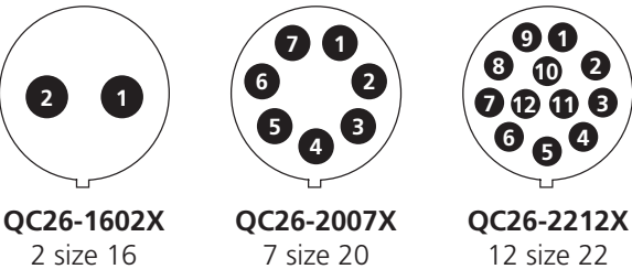
Plugs - cavity identification from rear
