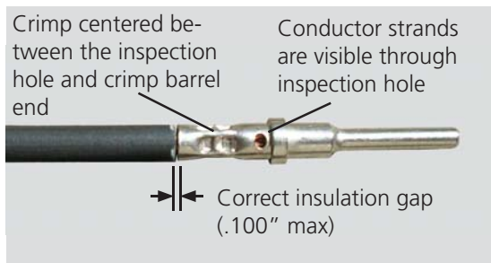
Acceptable Crimp
