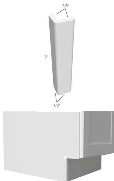
Toe Kick Cap Installed on Base Cabinet
