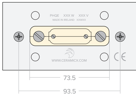
Element supplied with Wave Spring and Clip
