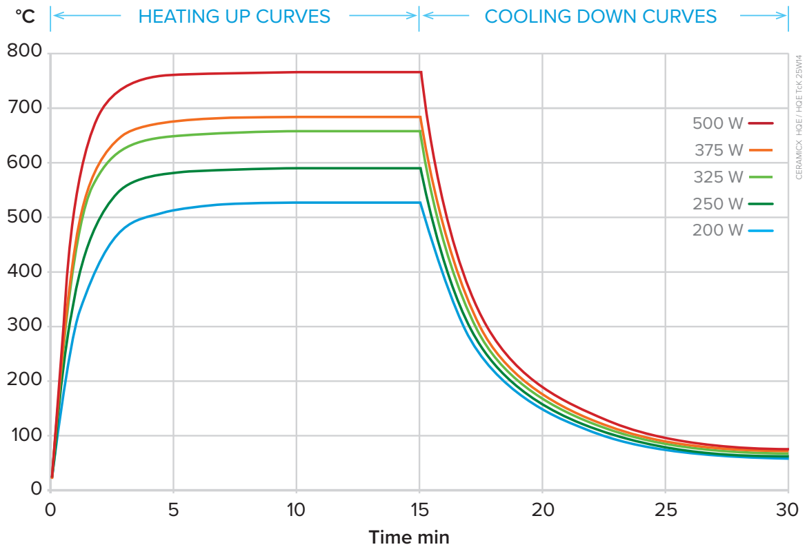
PHQE Heat up and cool down curves showing average surface temperature measured with a thermal imaging camera set to an emissivity of 0.7
