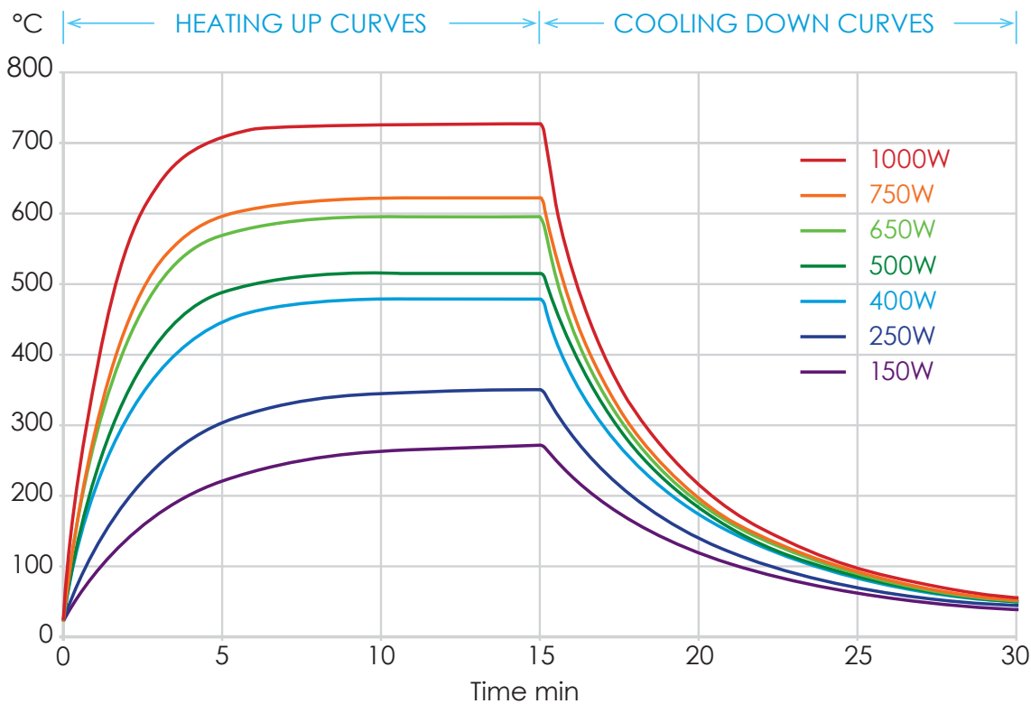
HTE Heat up and cool down curves showing average surface temperature measured with a thermal imaging camera set to an emissivity of 0.95 (element mounted in a polished aluminium clad steel reflector)
