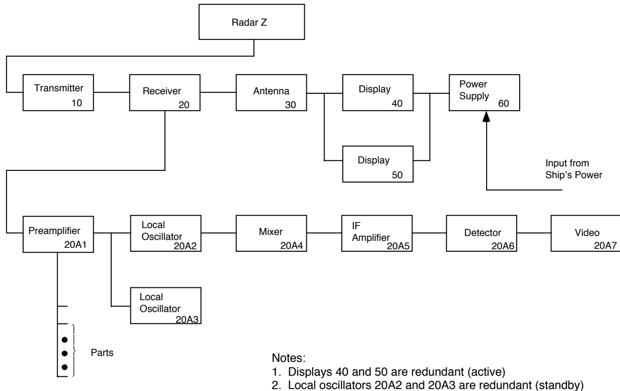
FIGURE 7.8-4: SYMBOLIC LOGIC DIAGRAM OF RADAR EXAMPLE
