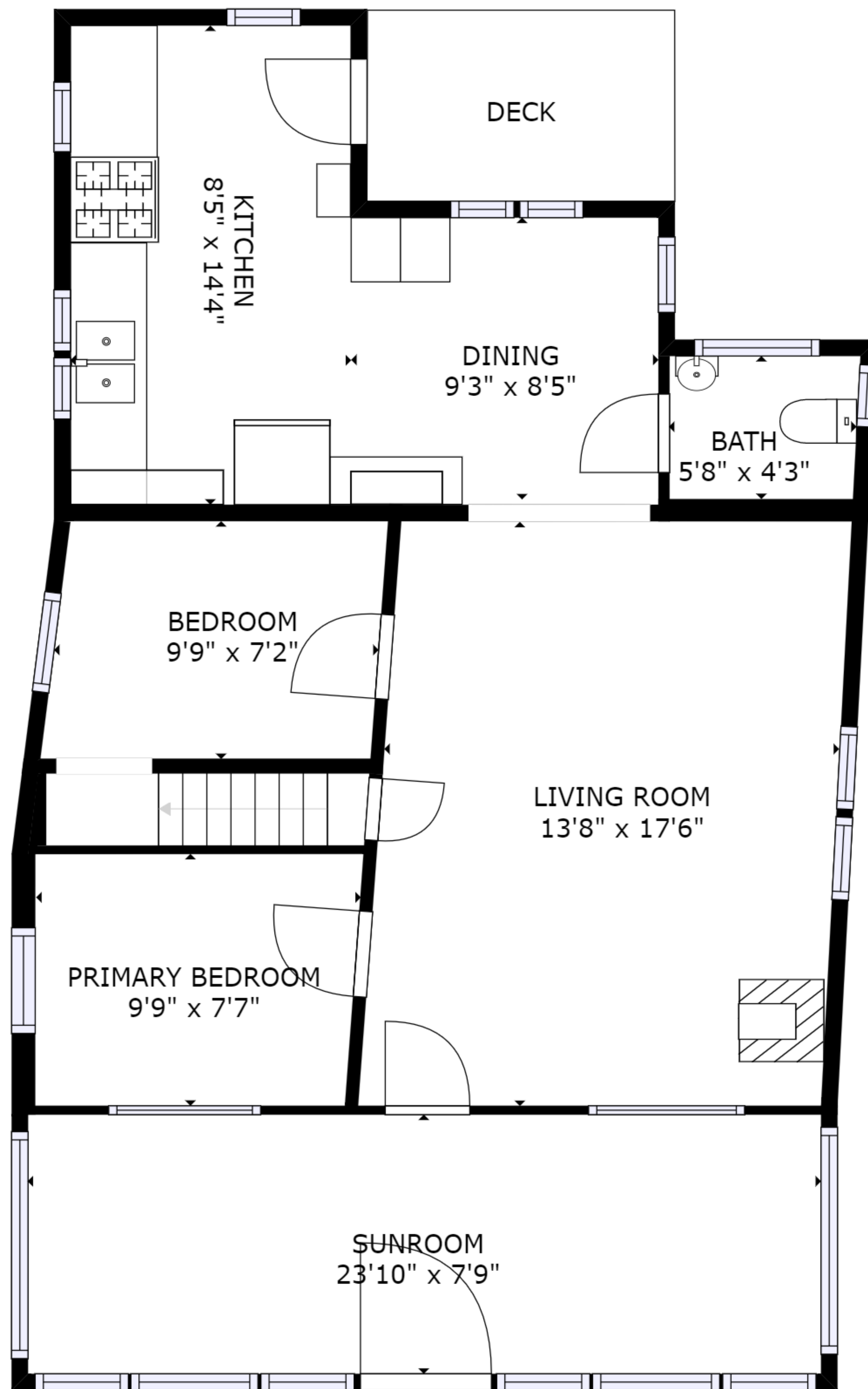
FLOOR 1
