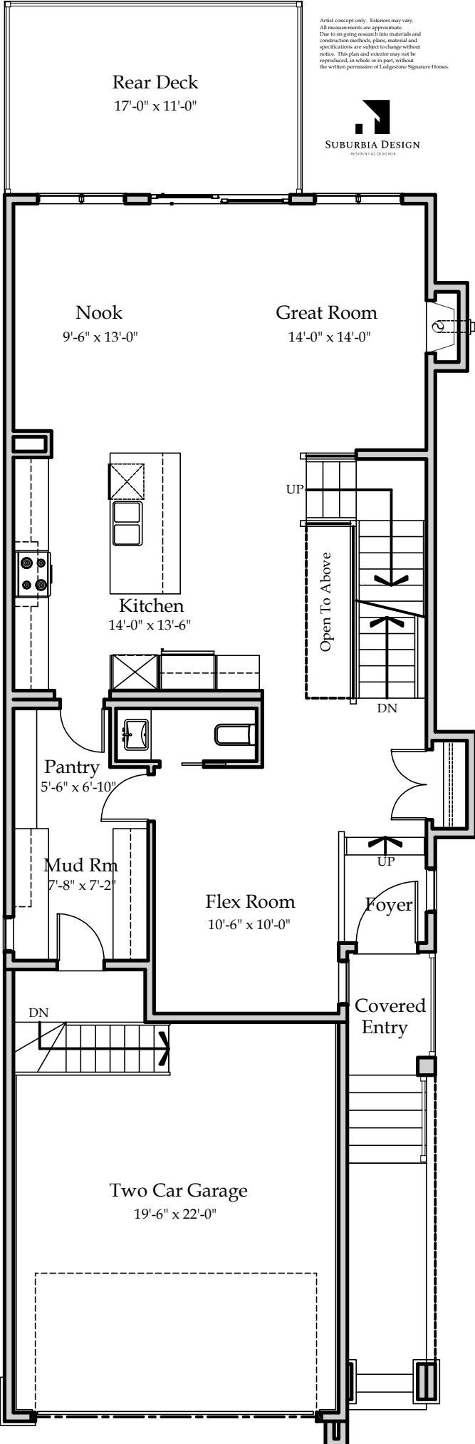
MAIN FLOOR PLAN @ 1,121 SQ.FT. TOTAL SQ.FT. @ 2,681
