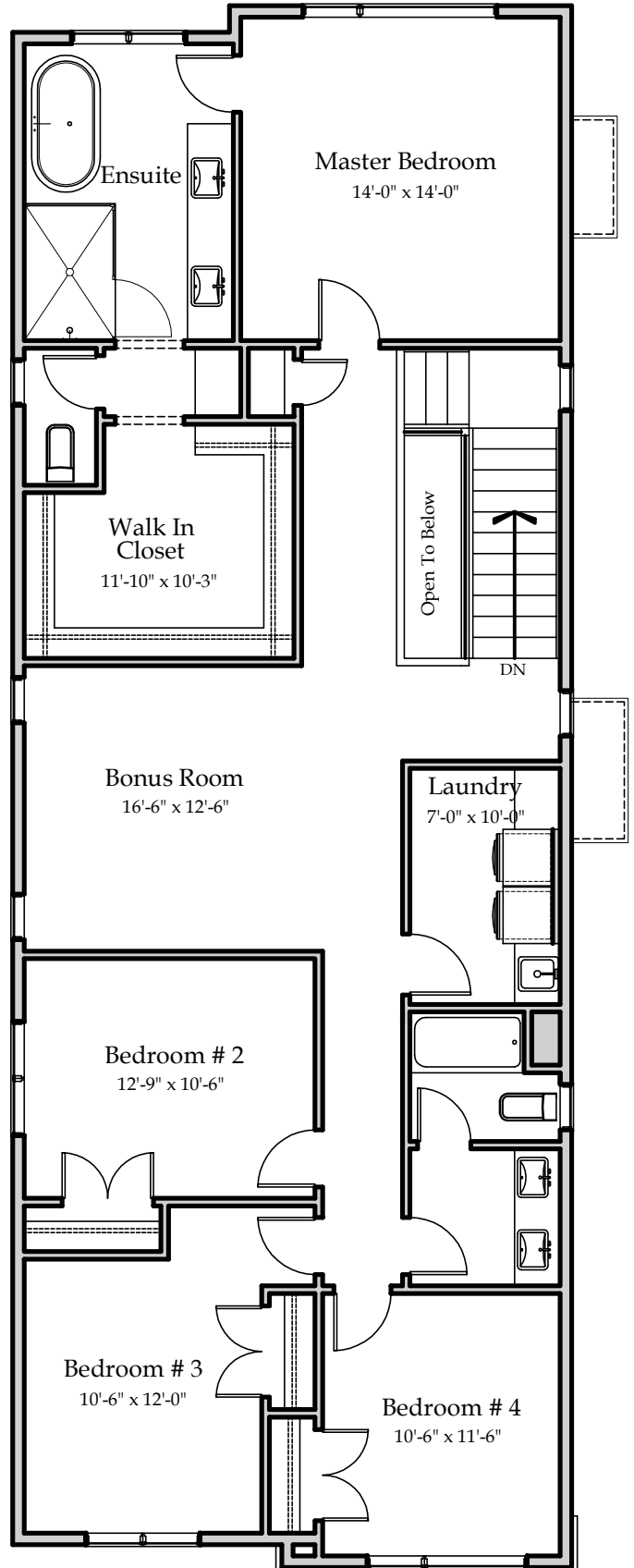
UPPER FLOOR PLAN @ 1,560 SQ.FT.
