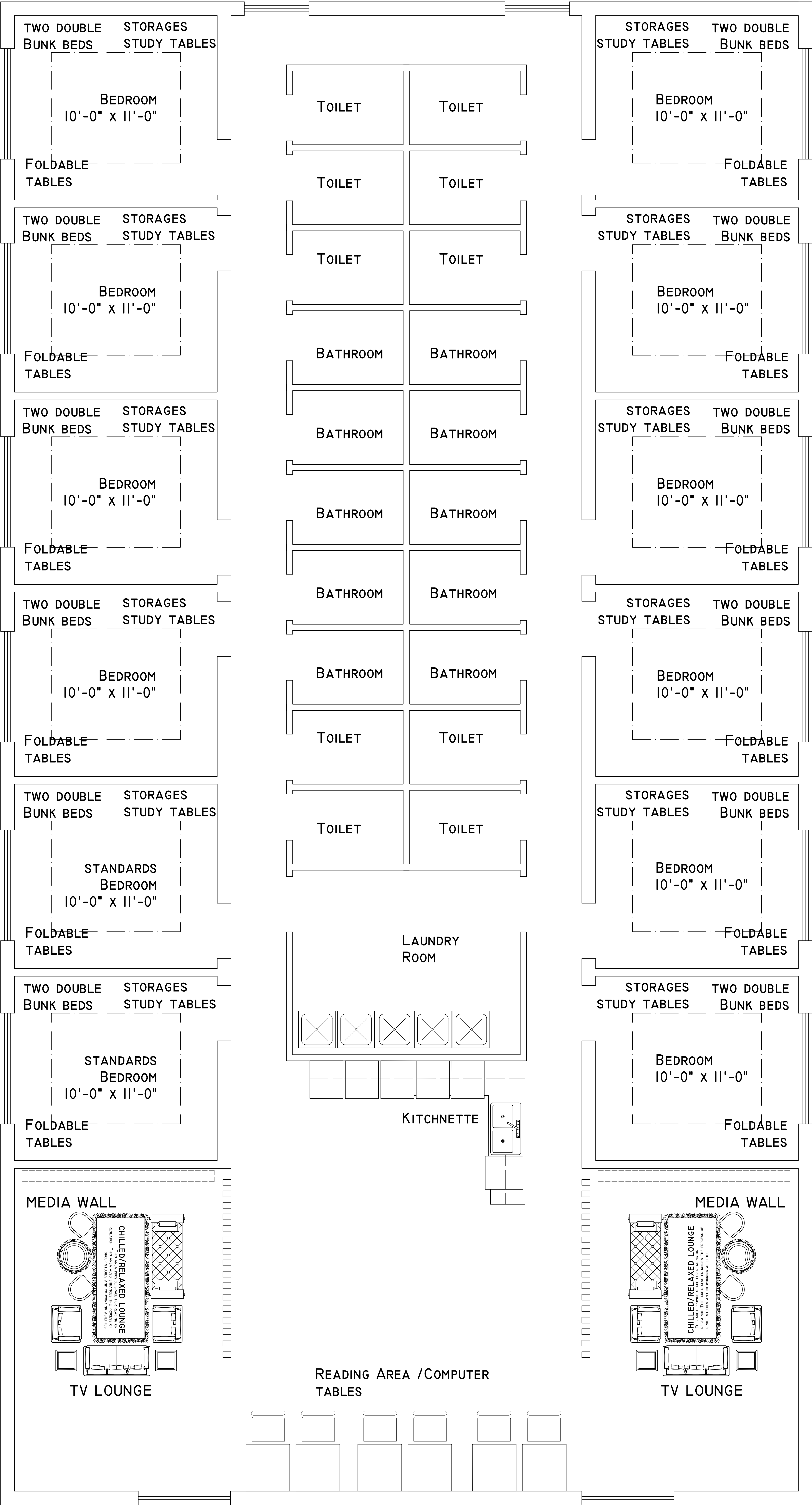
HOUSE FIRST FLOOR-PLAN AREA : 3200 SQFT
