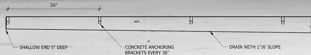
1 SLOT DRAIN SIDE VIEW Scale: 3/4" = 1'-0"
