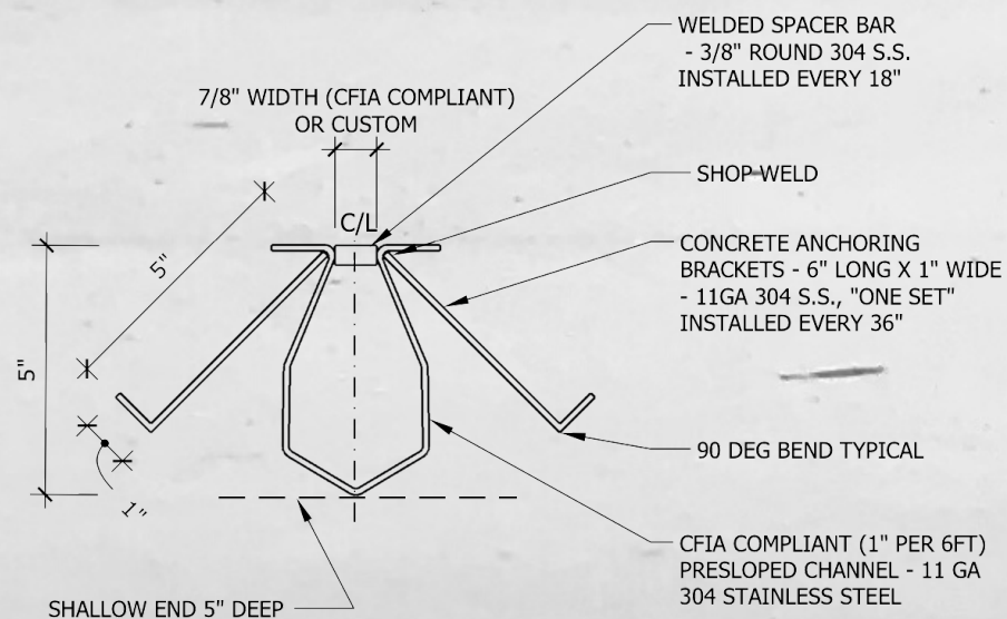
2 SLOT DRAIN FRONT VIEW Scale: 3" = 1'-0"
