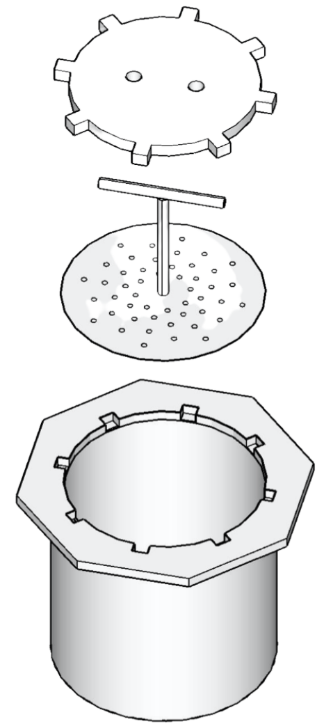
3 SUMP EXPLODED VIEW Scale: 1 1/2" = 1'-0"
