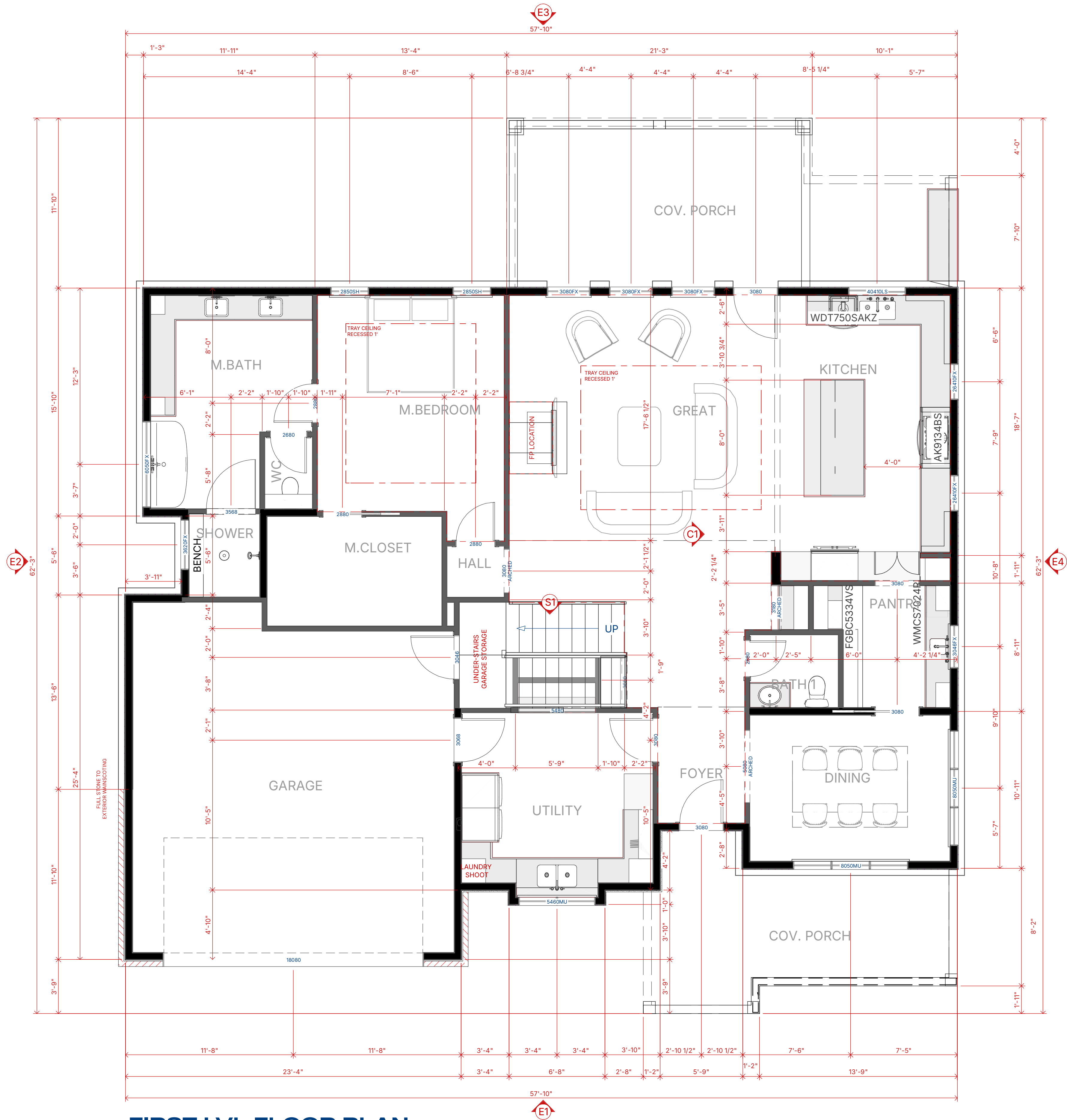
FIRST LVL FLOOR PLAN 1/4"=1'
