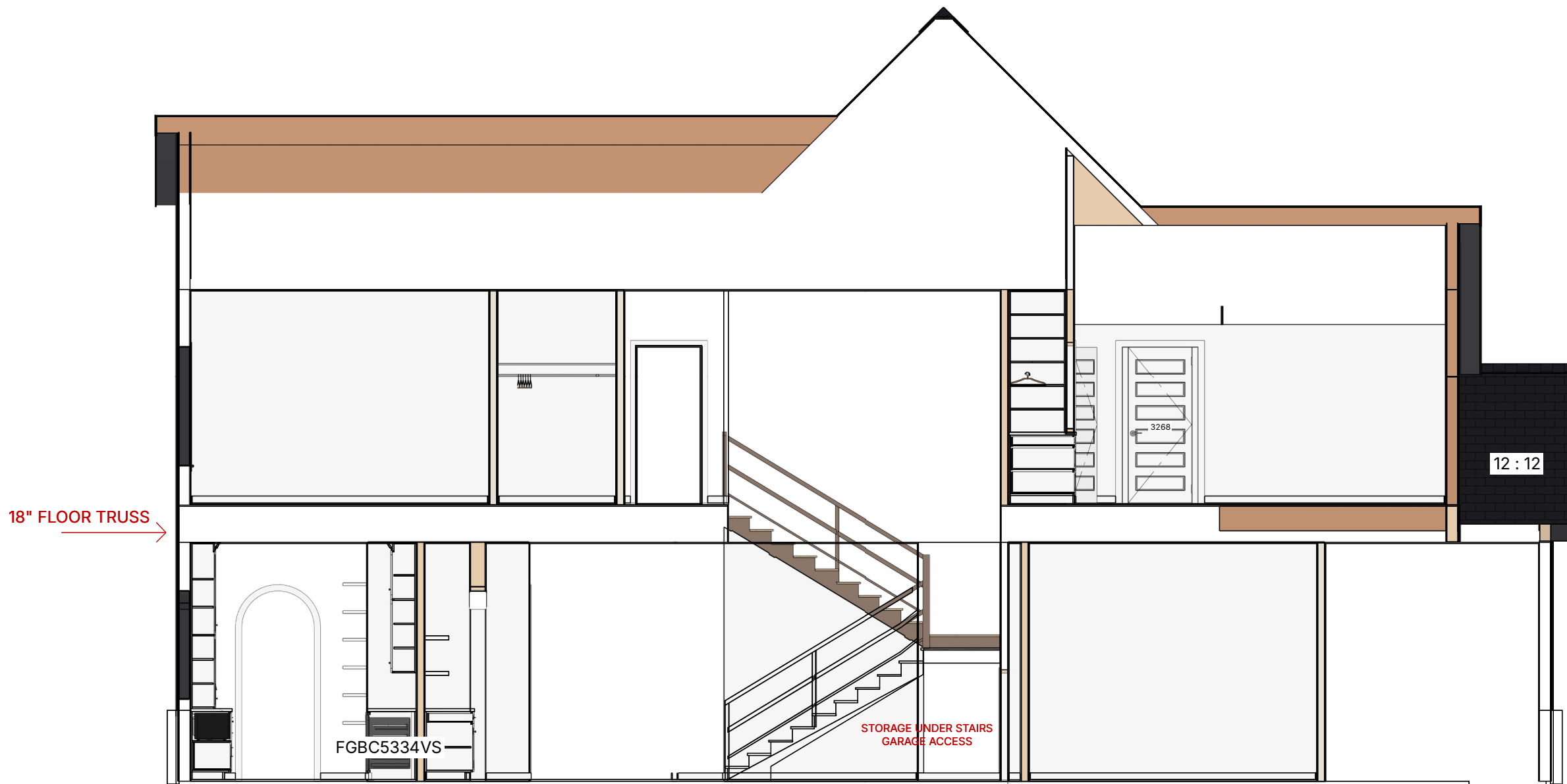
S1 CROSS SECTION 1 3/16 IN = 1 FT
