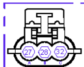
DETAIL L
