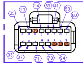
DETAIL I
